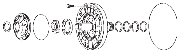
Oil Pump Assy
