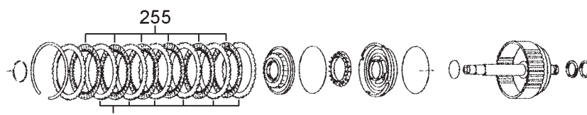
'C2' Clutch (5th, 6th, 7th, & 8th)
