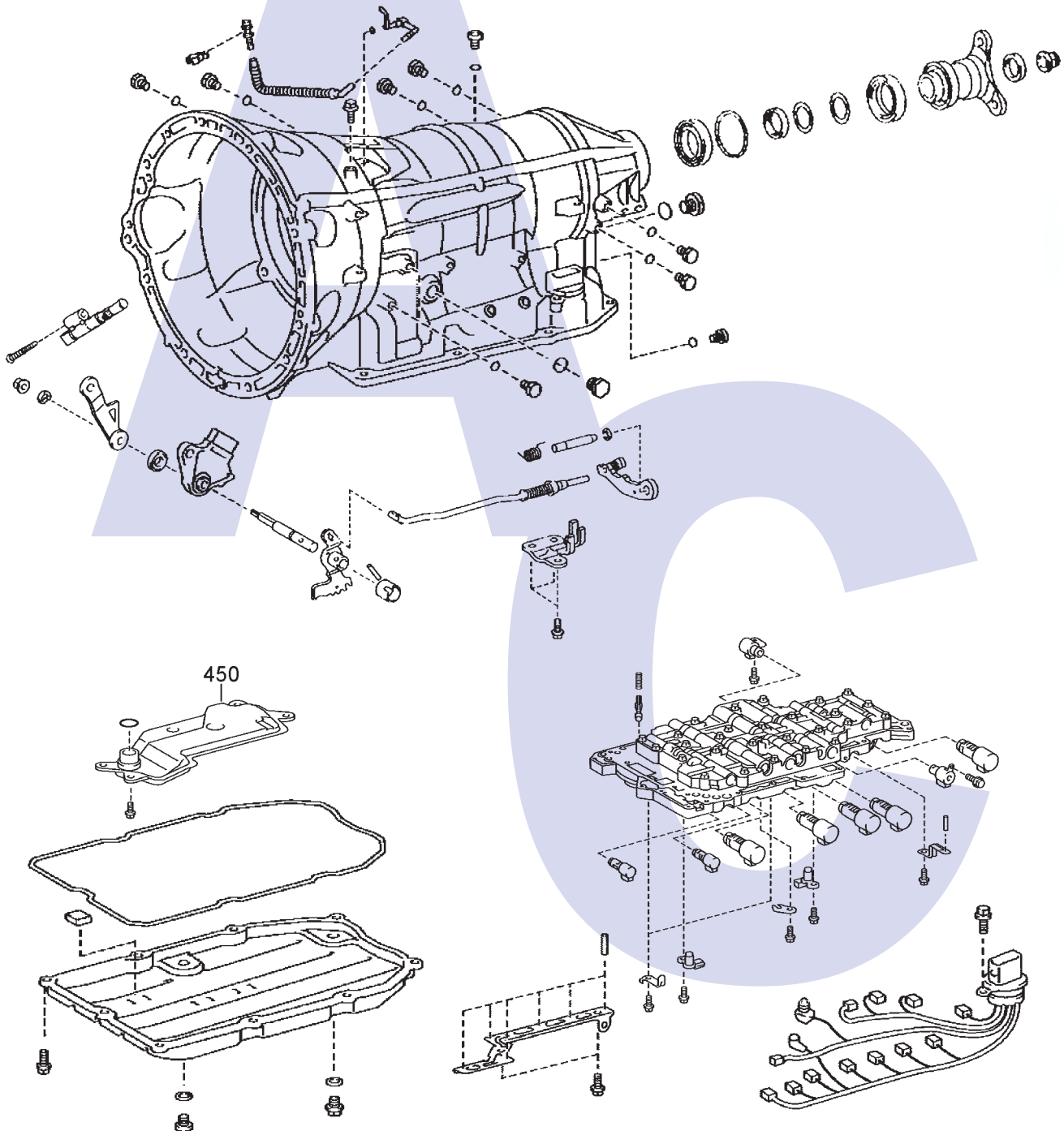
Main Casing, Filter, Oil Pan, Valve Body, Sensors & Loom
