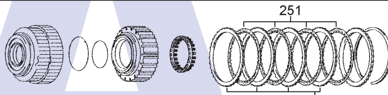
'C3' Clutch (3rd & 7th)
