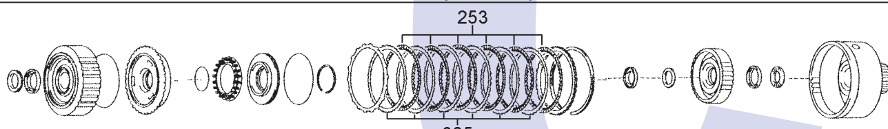
'C1' Clutch (1st, 2nd, 3rd, 4th & 5th)
