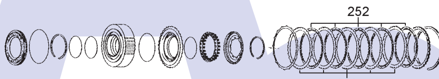
'C4' Clutch (Rev, 4th & 6th)
