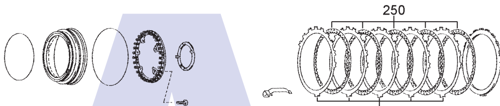
'B1' Brake (2nd & 7th)
